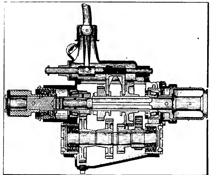
Fig. 10—Section through the gearset of Reo the Fifth
